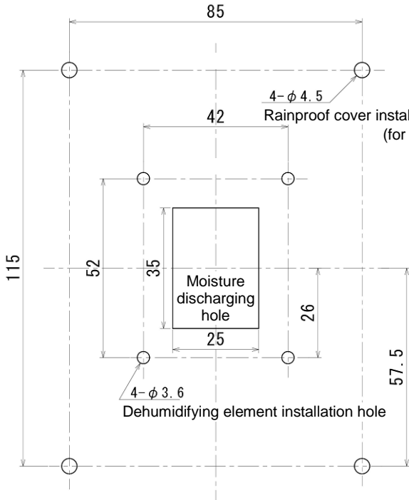
Fig.1 Installation dimensions
