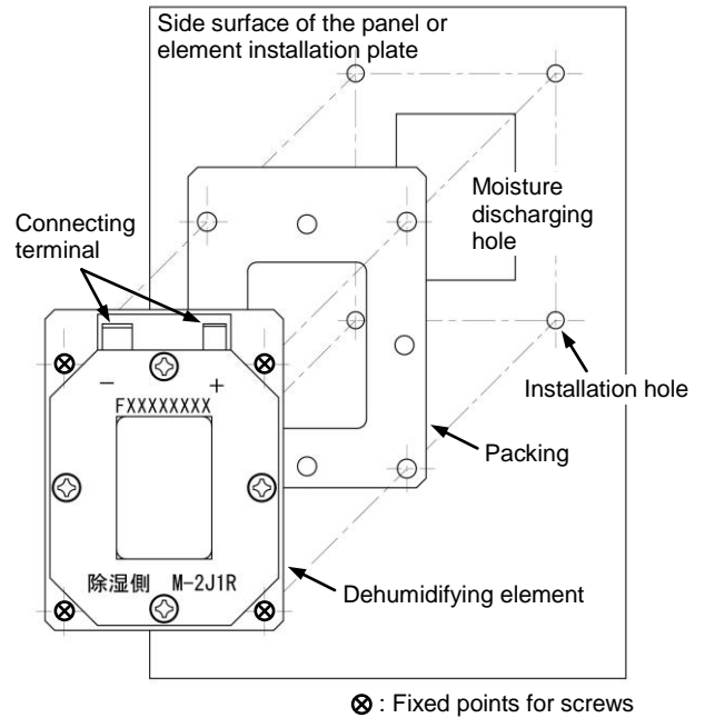
Fig.2 Installation method
