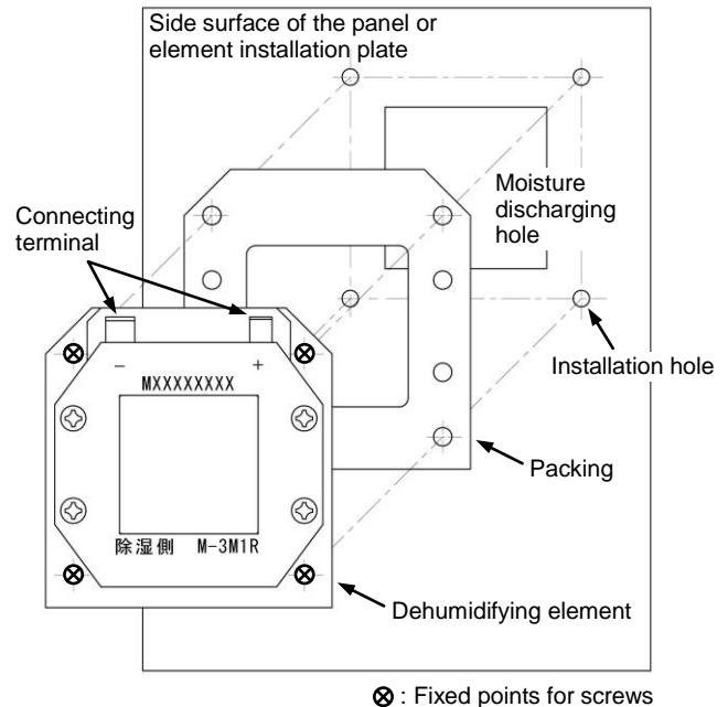
Fig.2 Installation method
