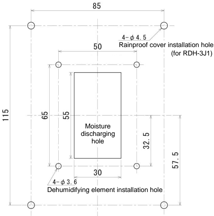
Fig.1 Installation dimensions
