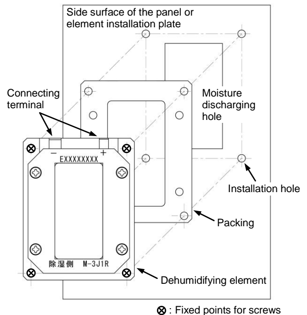
Fig.2 Installation method
