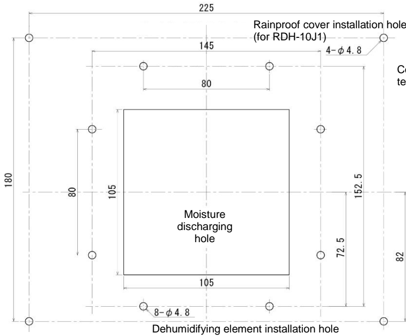
Fig.1 Installation dimensions
