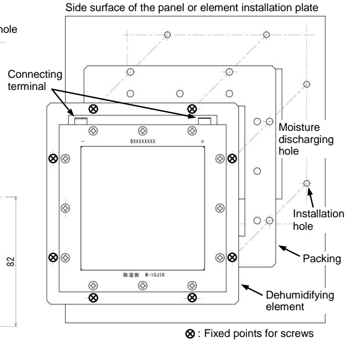
Fig.2 Installation method
