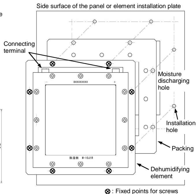
Fig.2 Installation method
